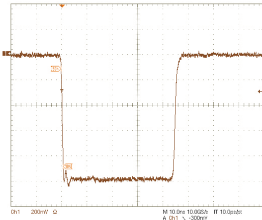
Figure: Current monitor output, scale: -0.4 A/Div
